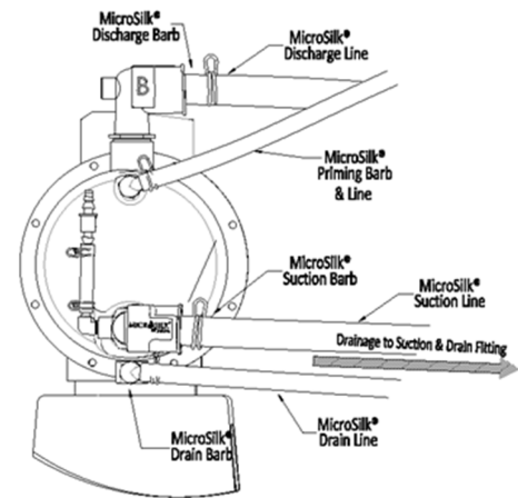
MicroSilk® Pump Connections Figure 11
