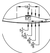
Faucet Deck Flat Dimensions
