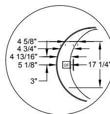
Faucetry Deck Flat Dimensions
