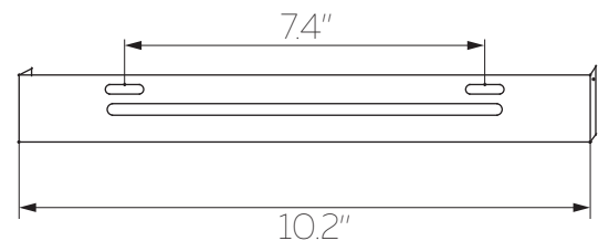
UPPER BRACKET
