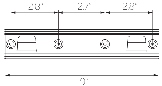
LOWER BRACKET
