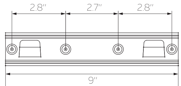
LOWER BRACKET
