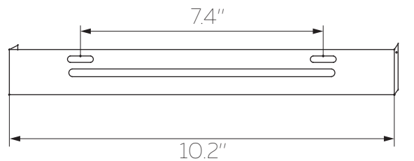
UPPER BRACKET
