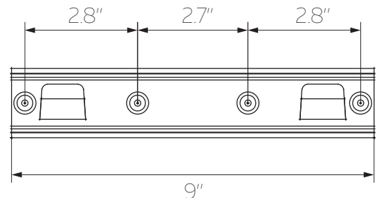
LOWER BRACKET
