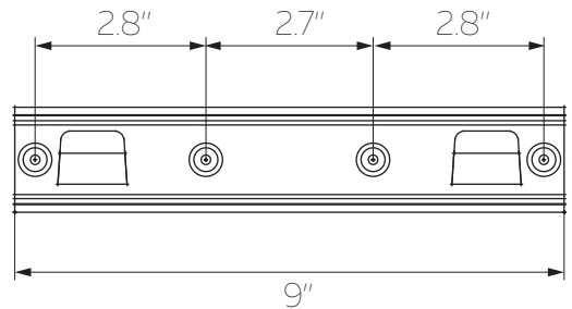
LOWER BRACKET
