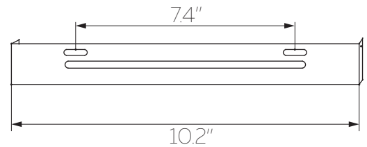
UPPER BRACKET
