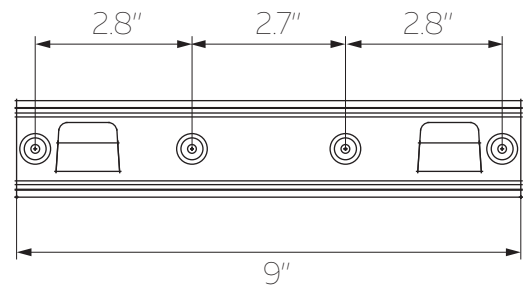
LOWER BRACKET
