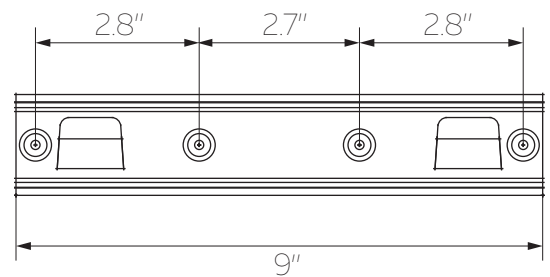
LOWER BRACKET
