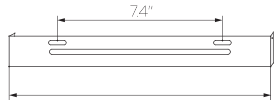
UPPER BRACKET
