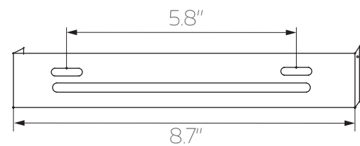
UPPER BRACKET
