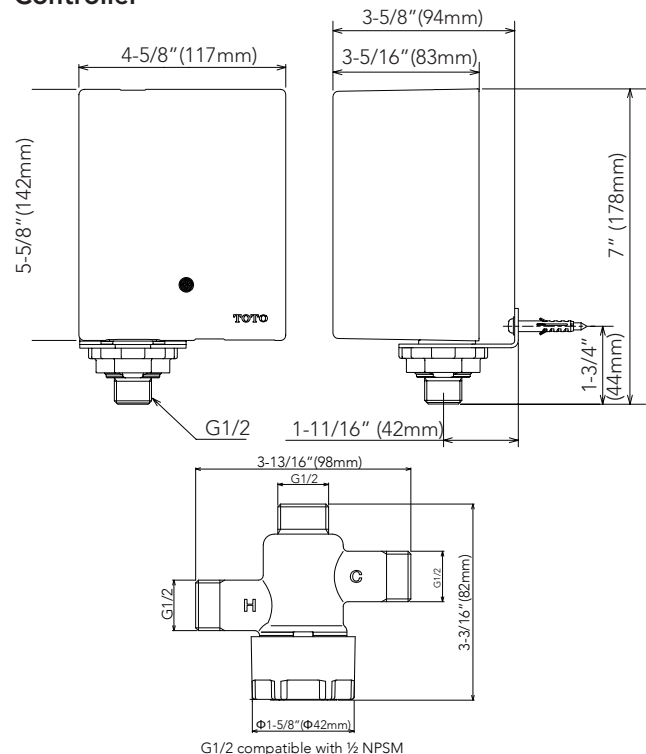
Thermostatic Mixing Valve (TLT10R)
